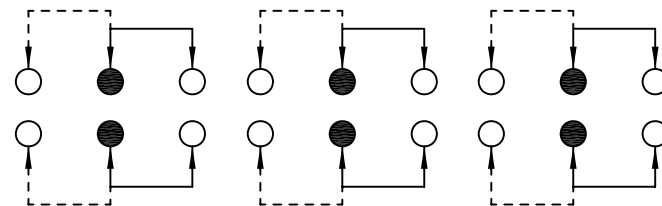
SCHEMATIC (SHORTING)
